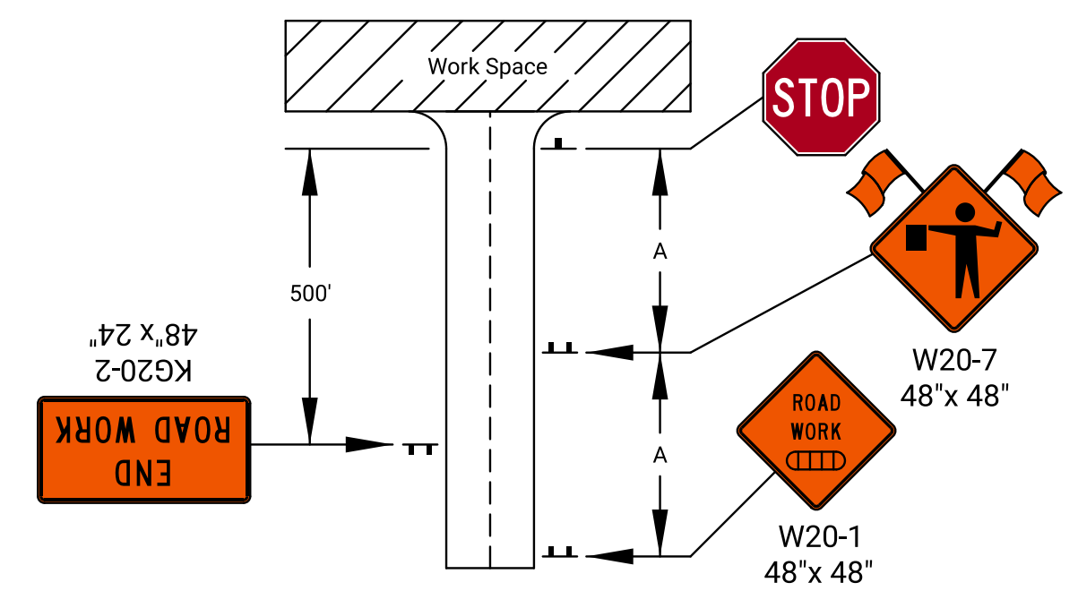
TYPICAL SIGNING FOR HIGHWAY OR MAJOR COLLECTOR APPROACH TO WORK SPACE
