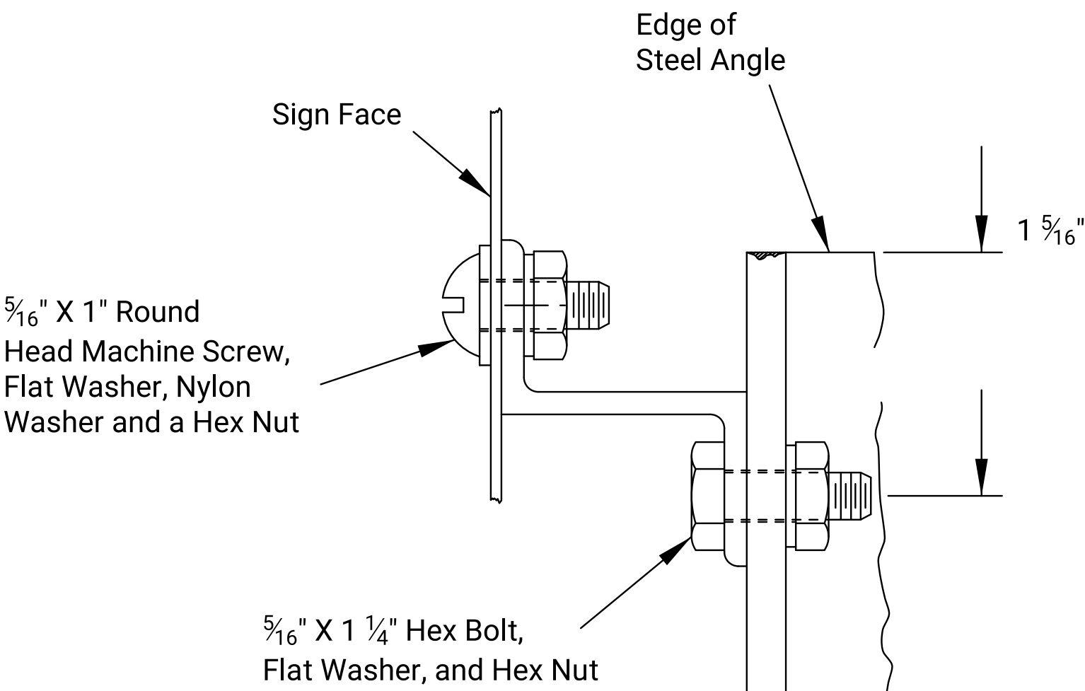
INSET AA
