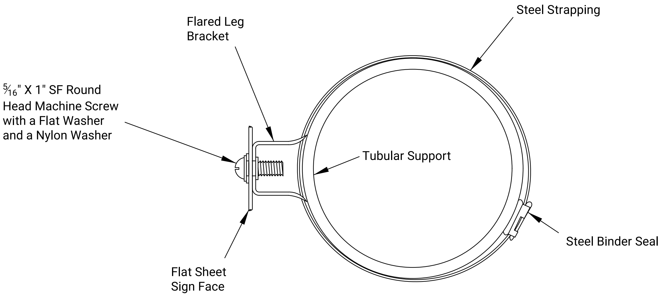
SECTION BB
