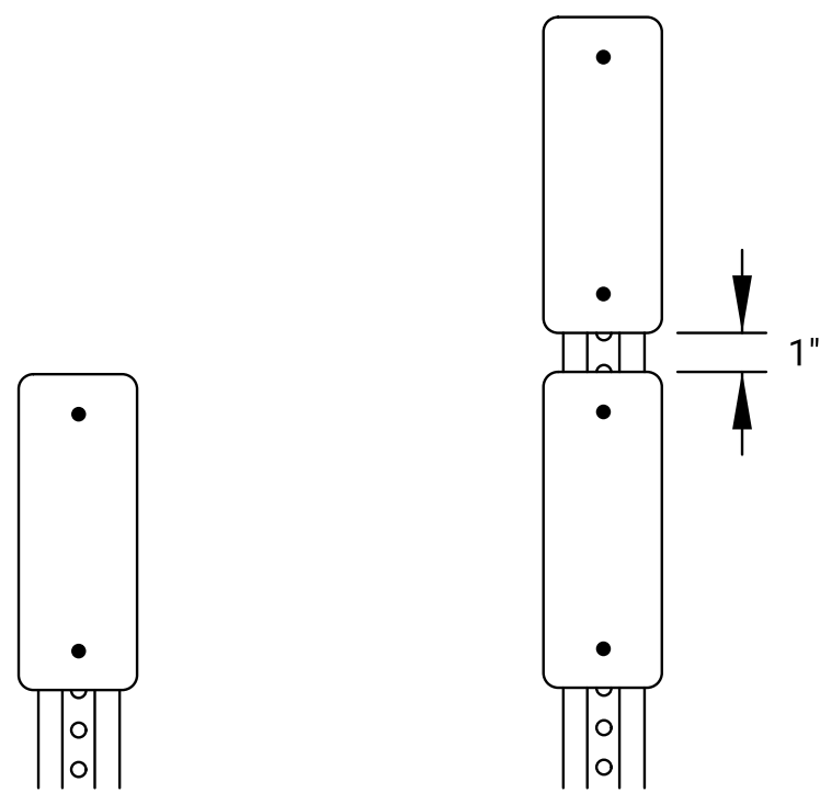
TYPICAL DELINEATOR ASSEMBLY
