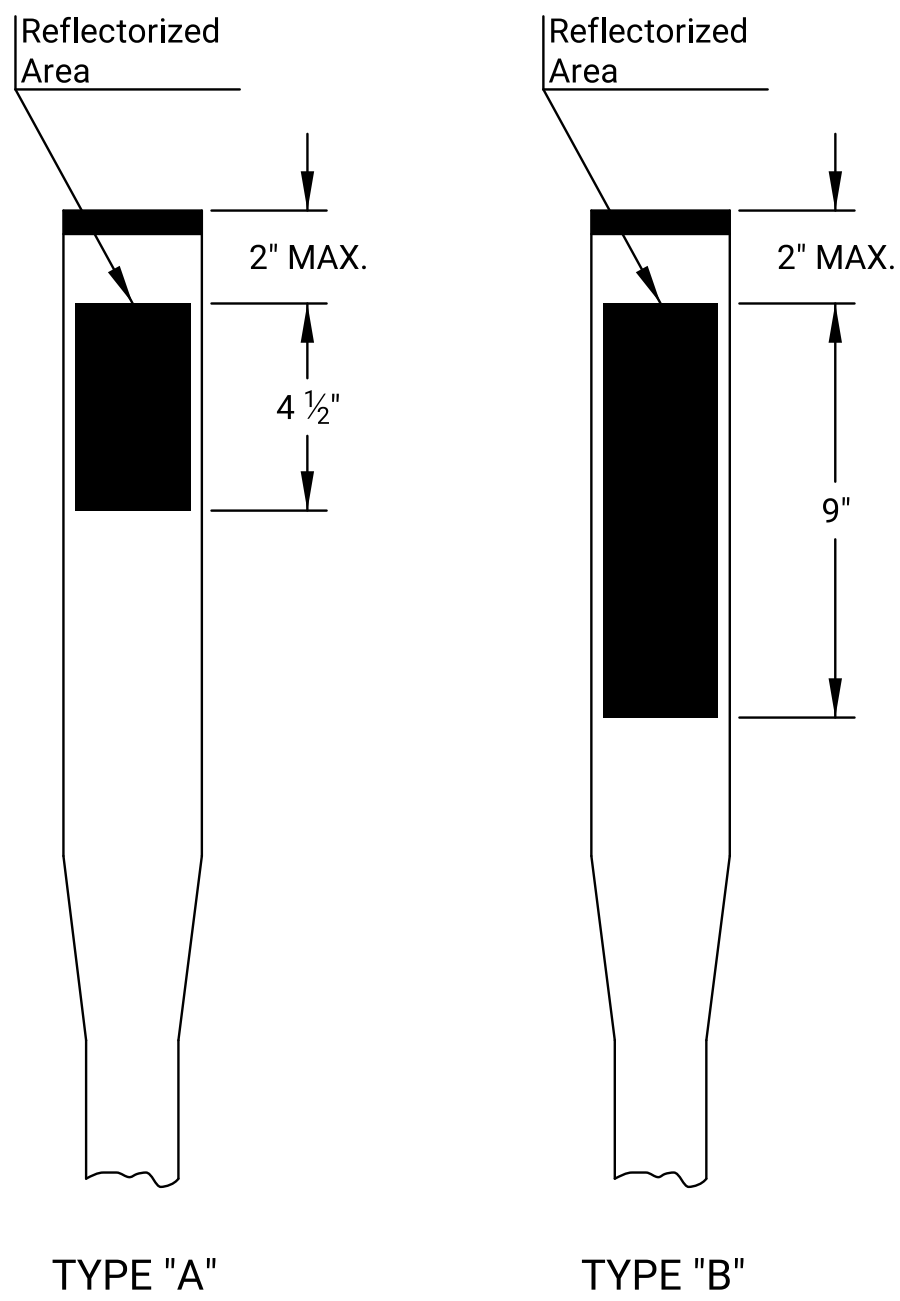
REFLECTORIZED AREA POSITIONING
