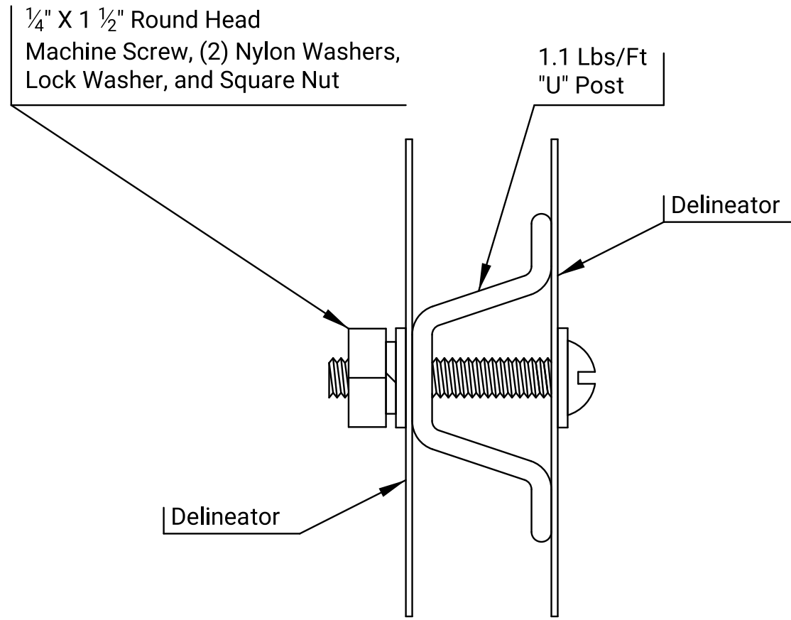
MOUNTING DETAILS (BACK TO BACK)
