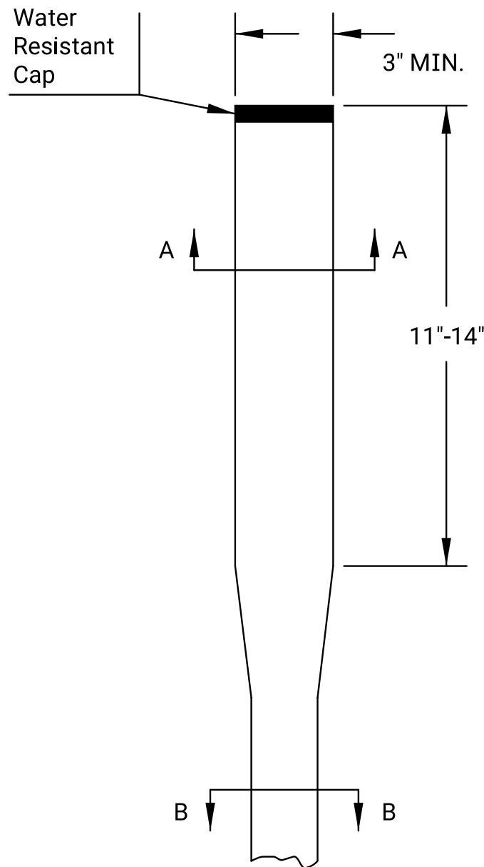
FLEXIBLE DELINEATOR POST DETAILS
