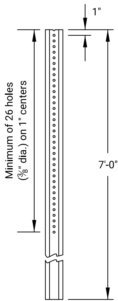
PUNCHING DETAILS
