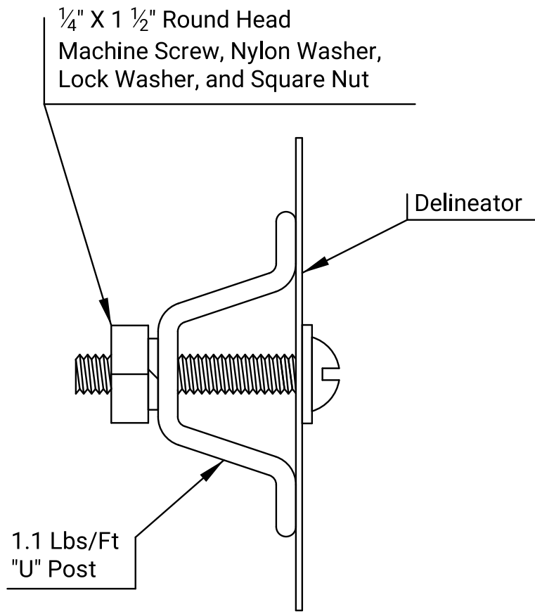
MOUNTING DETAILS (TYPICAL)
