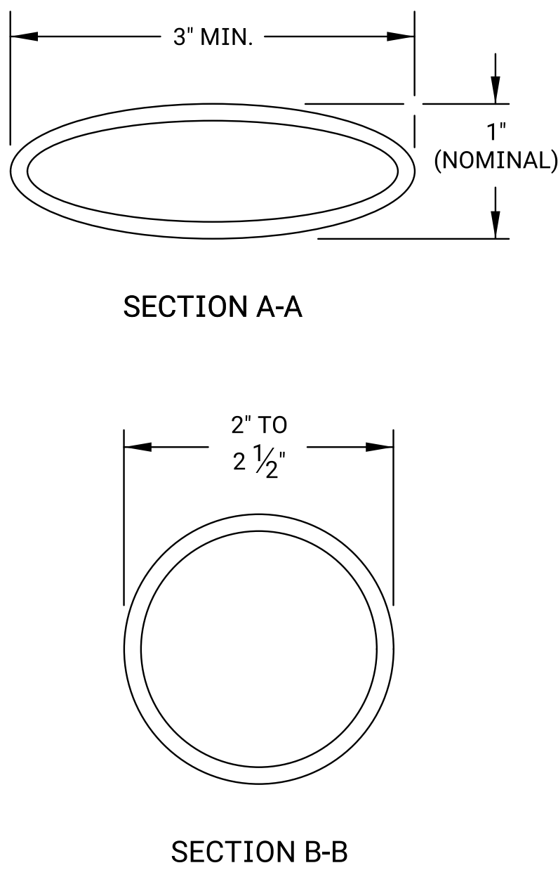
FLEXIBLE DELINEATOR POST DETAILS
