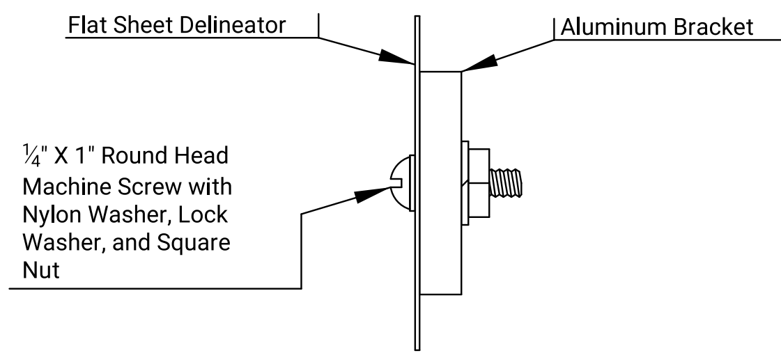
DETAILS FOR ATTACHING DELINEATOR TO BRACKET
