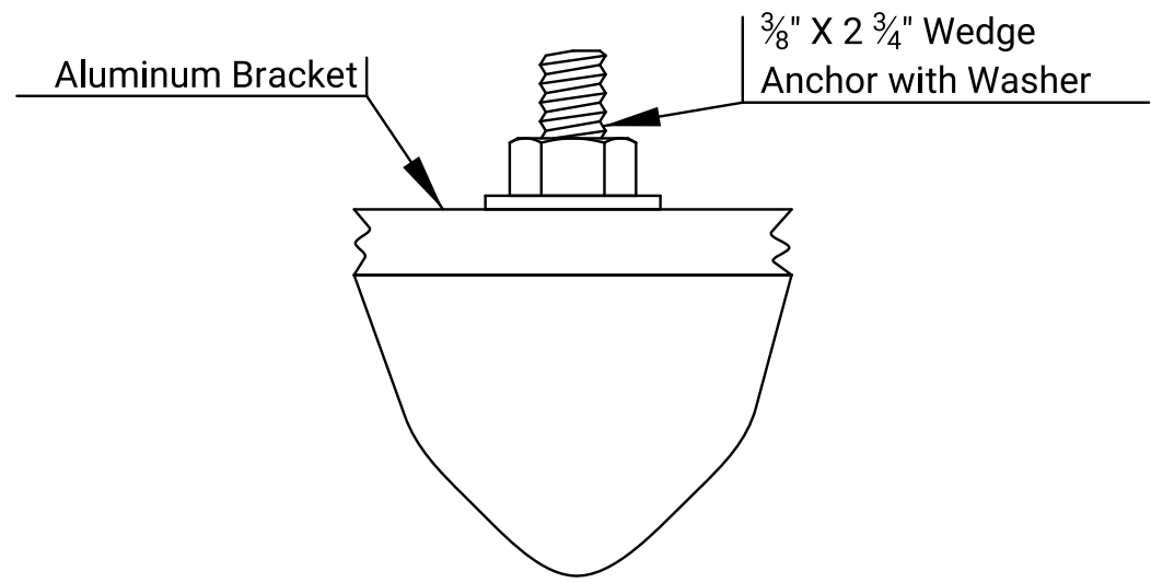
DETAILS FOR ATTACHING BRACKET TO CONCRETE SURFACE
