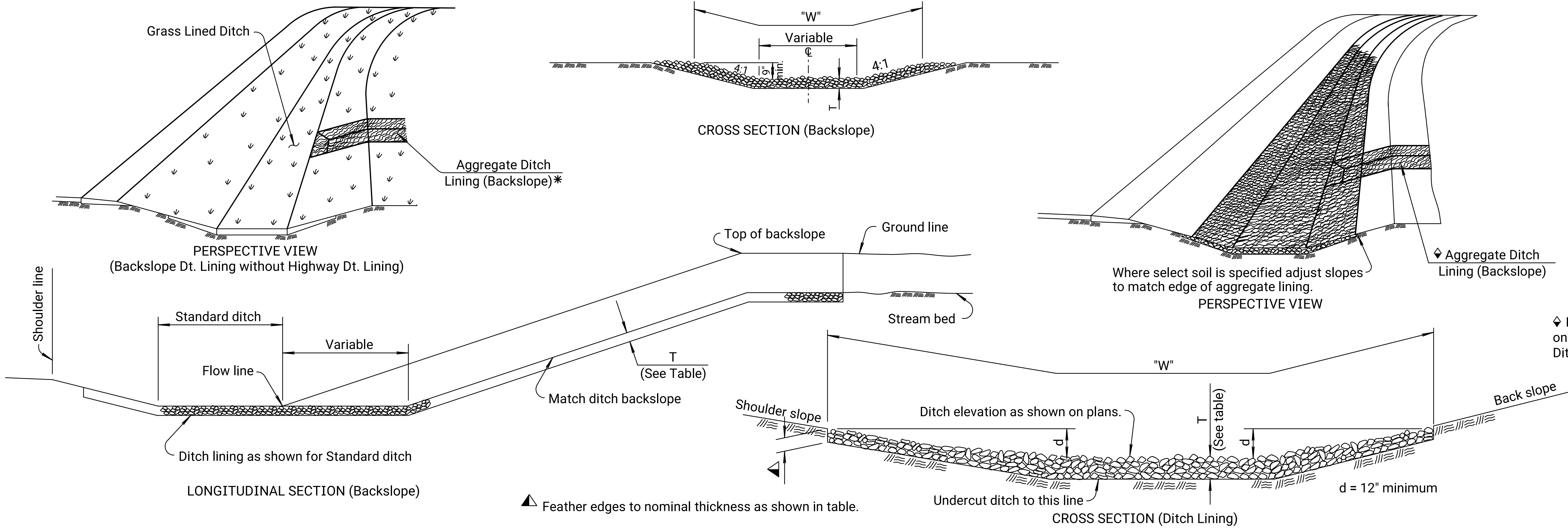
AGGREGATE DITCH LINING (D 50 )
