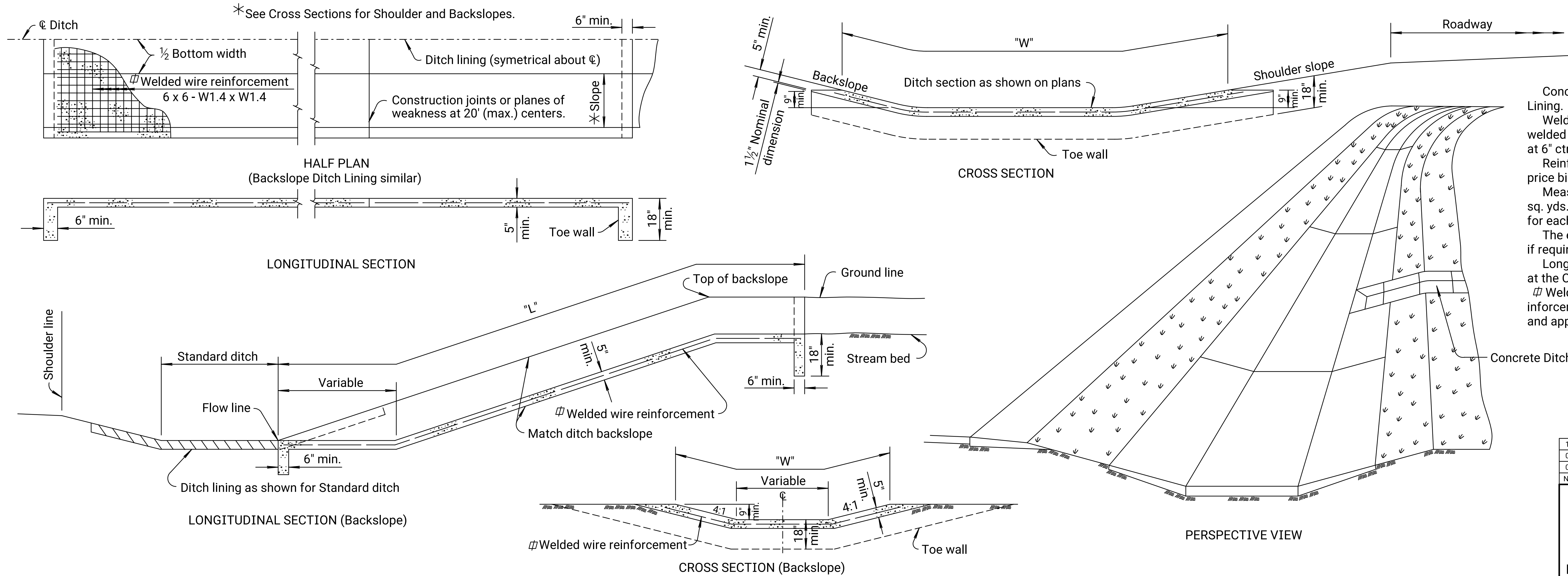
CONCRETE DITCH LINING
