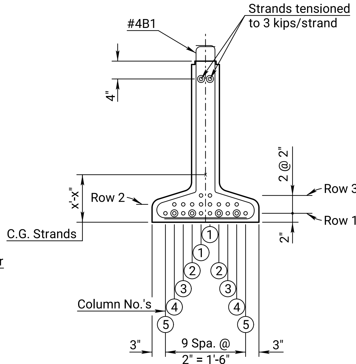
STRAND SPACING
