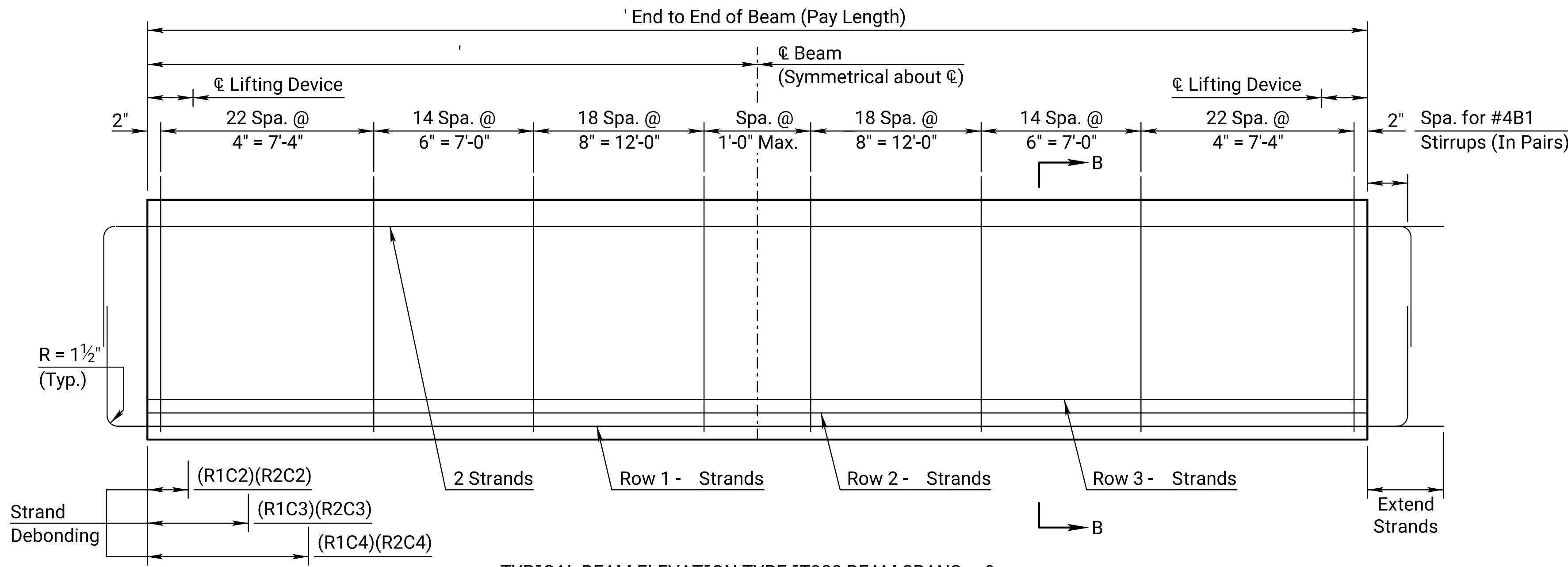
TYPICAL BEAM ELEVATION TYPE IT900 BEAM SPANS &
