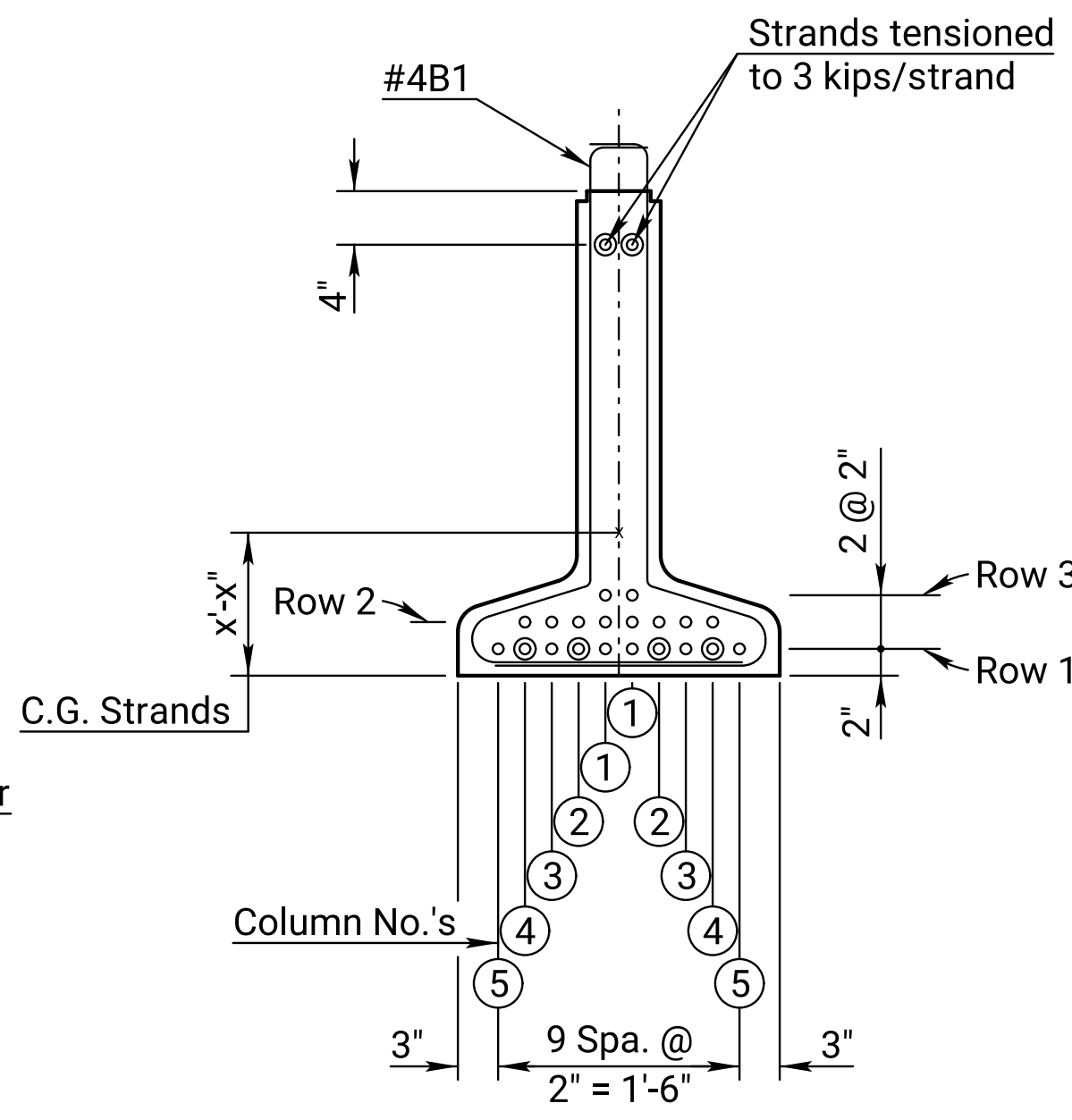
STRAND SPACING
