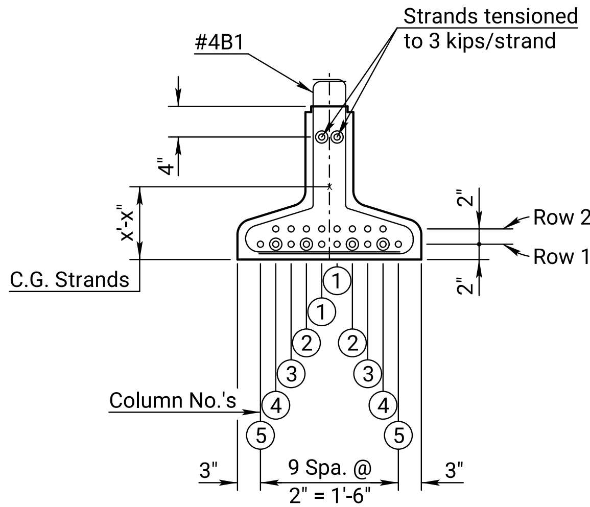
STRAND SPACING
