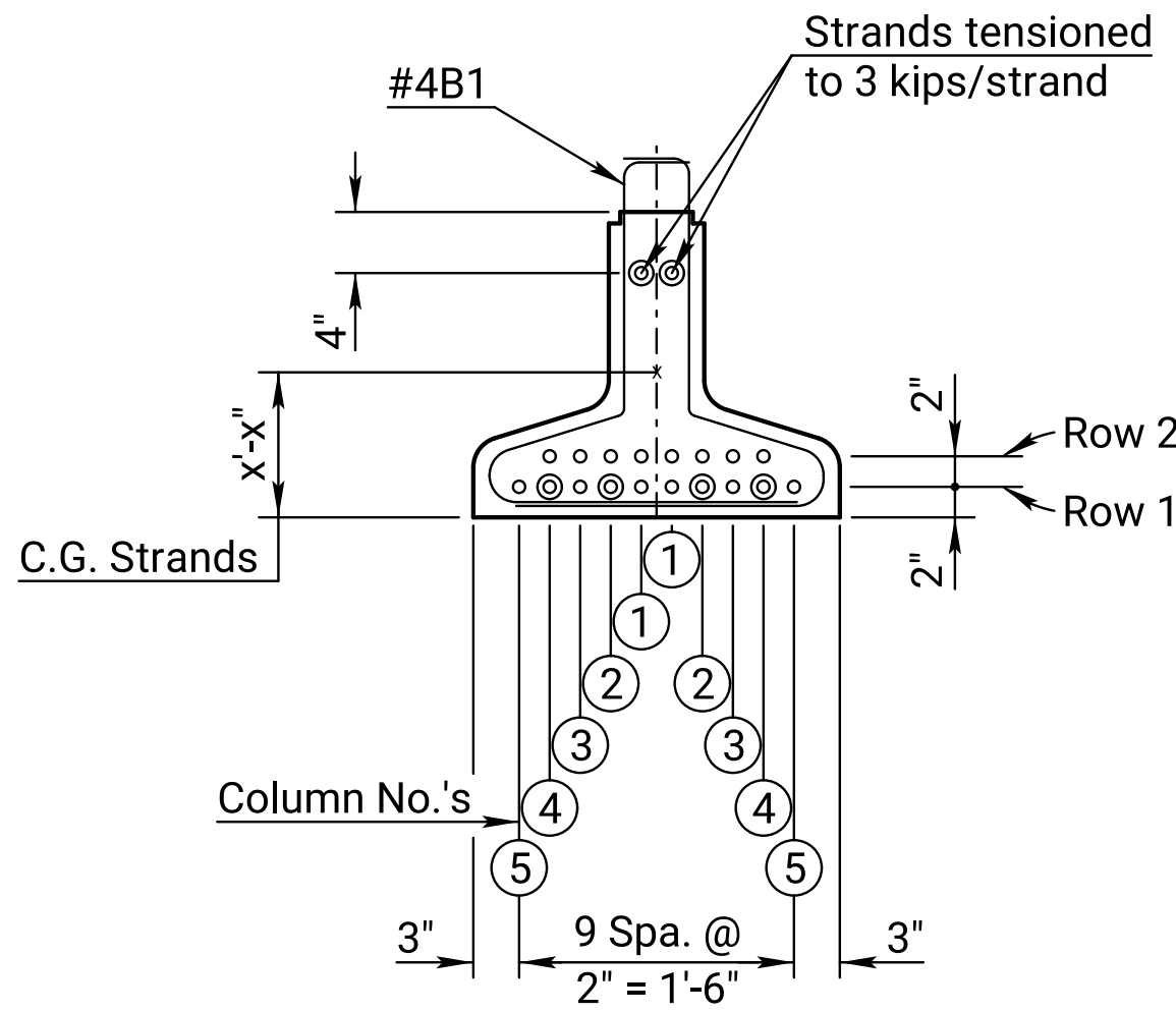
STRAND SPACING
