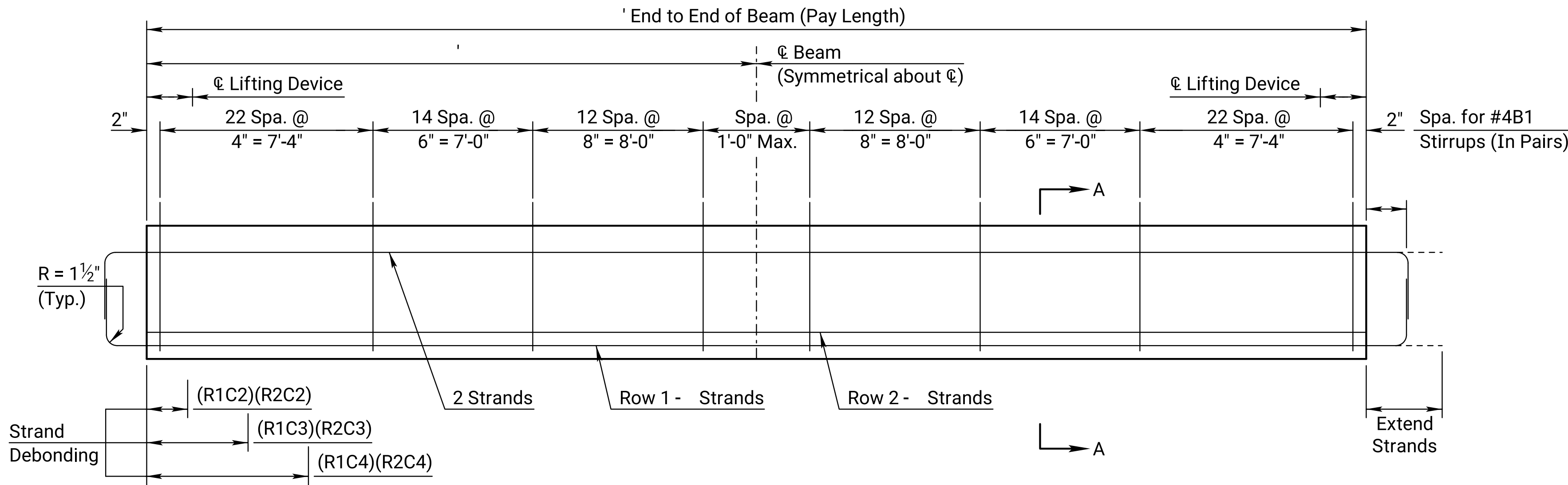
TYPICAL BEAM ELEVATION TYPE IT500 BEAM SPANS &
