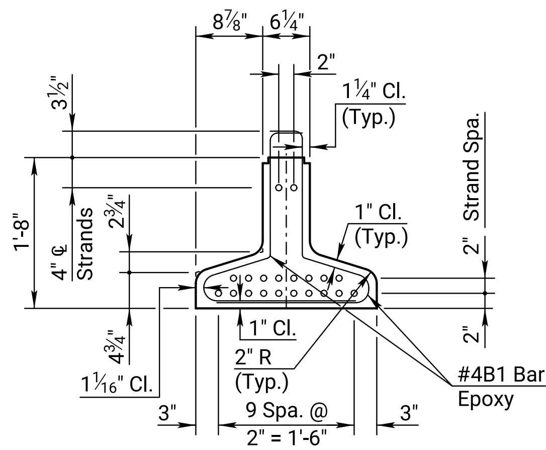
SECTION B-B
