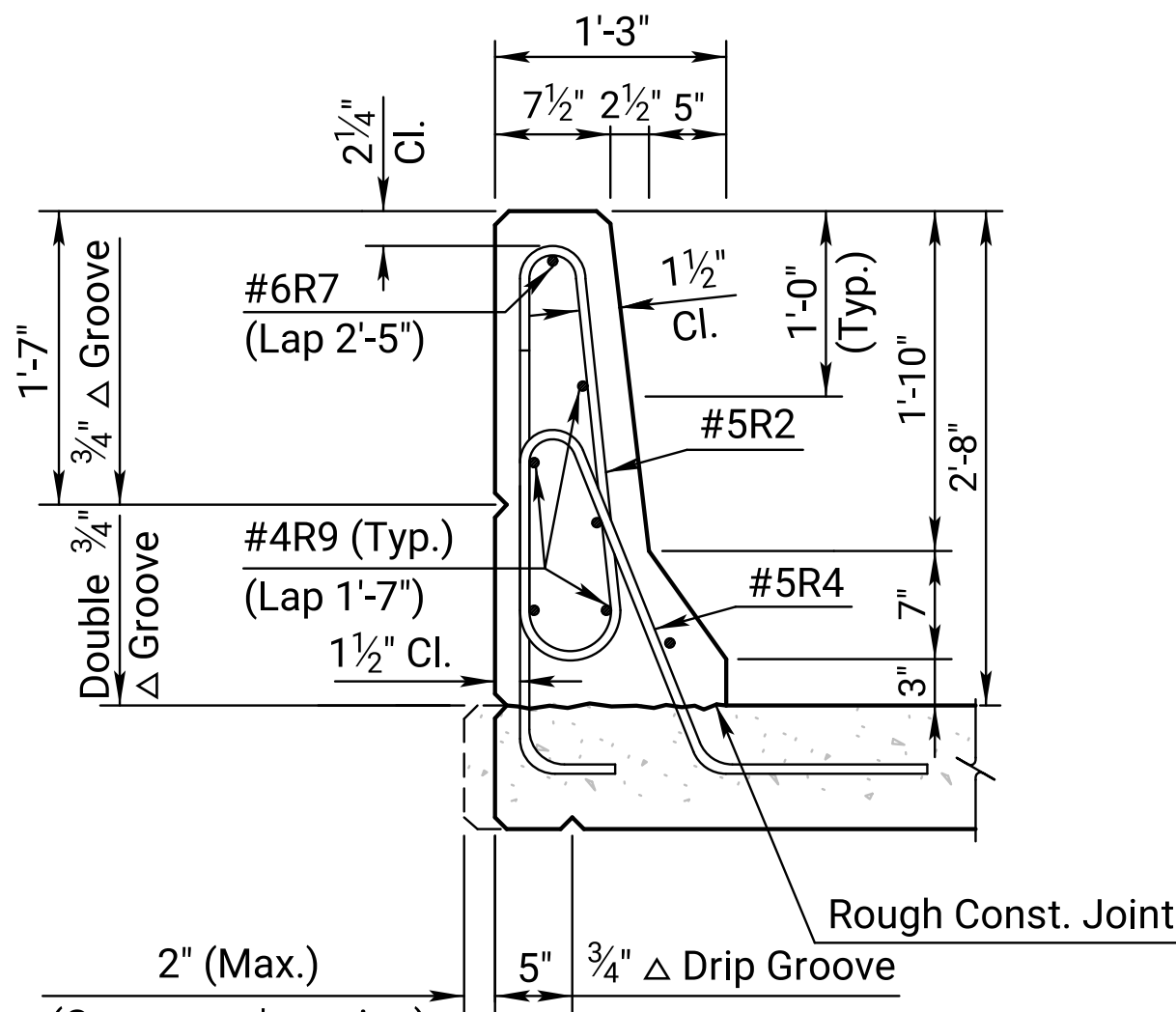
SECTION THRU BARRIER
