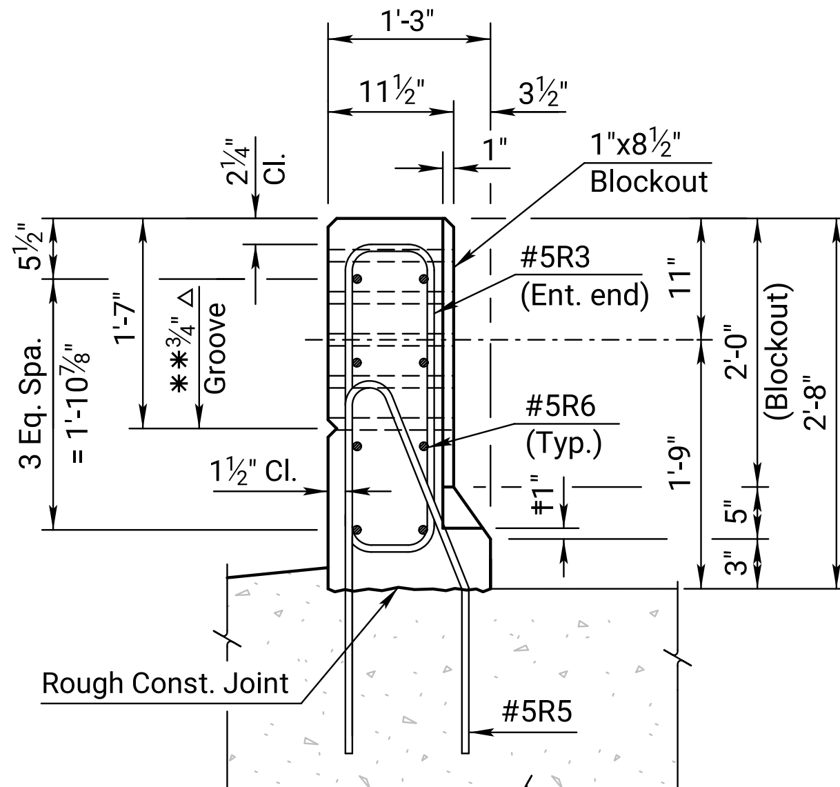
SECTION THRU BARRIER ENTRANCE TYPE END (At abutment)
