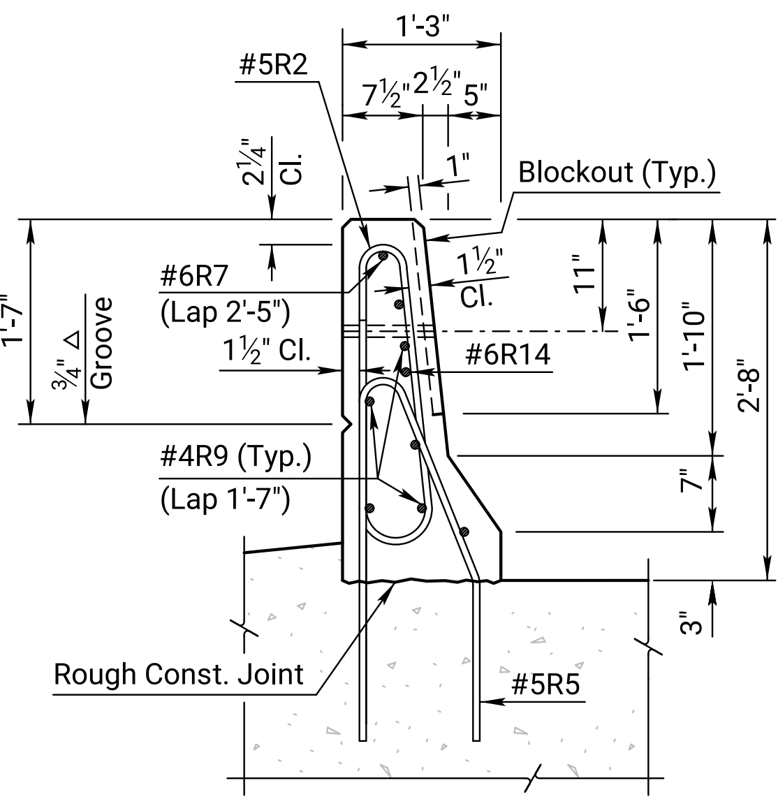
SECTION THRU BARRIER EXIT TYPE END (At abutment)
