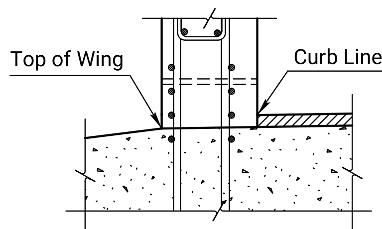
DETAIL A
