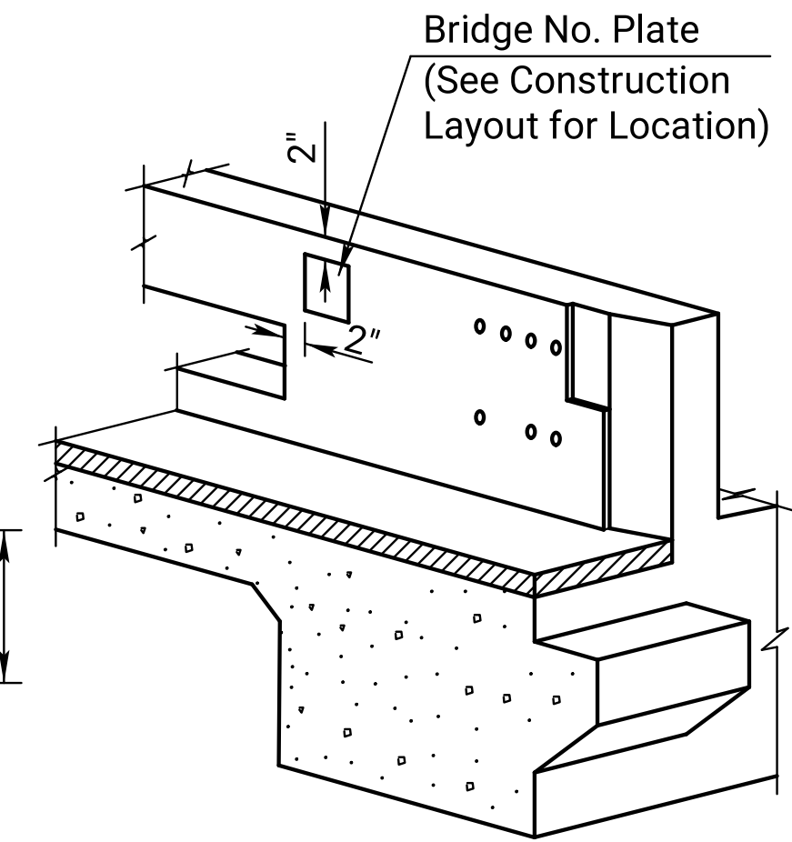
BRIDGE NUMBER PLATE PLACEMENT DETAIL (If Required)
