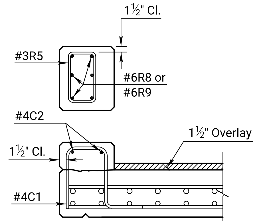
TYPICAL SECTION BETWEEN POSTS
