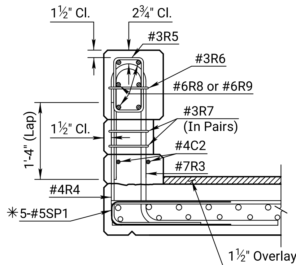
TYPICAL INTERIOR POST SECTIONS
