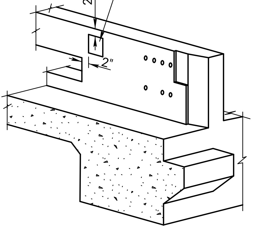
BRIDGE NUMBER PLATE PLACEMENT DETAIL (If Required)
