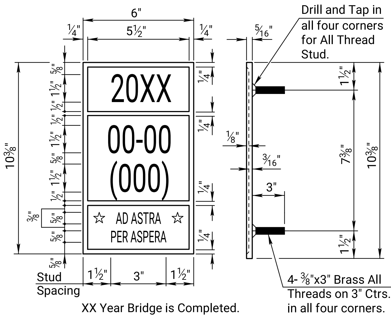
XX Year Bridge is Completed. in all four corners. BRIDGE NUMBER PLATE (1 Required) (See Construction Layout for Location)
