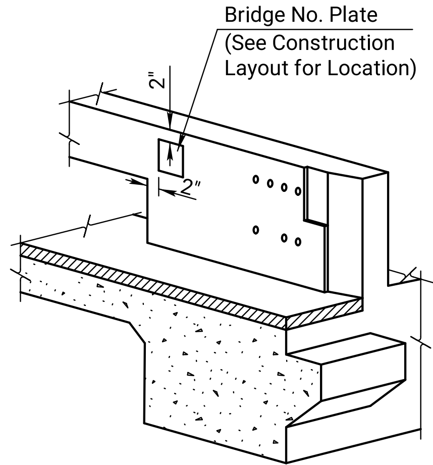
BRIDGE NUMBER PLATE PLACEMENT DETAIL (If Required)
