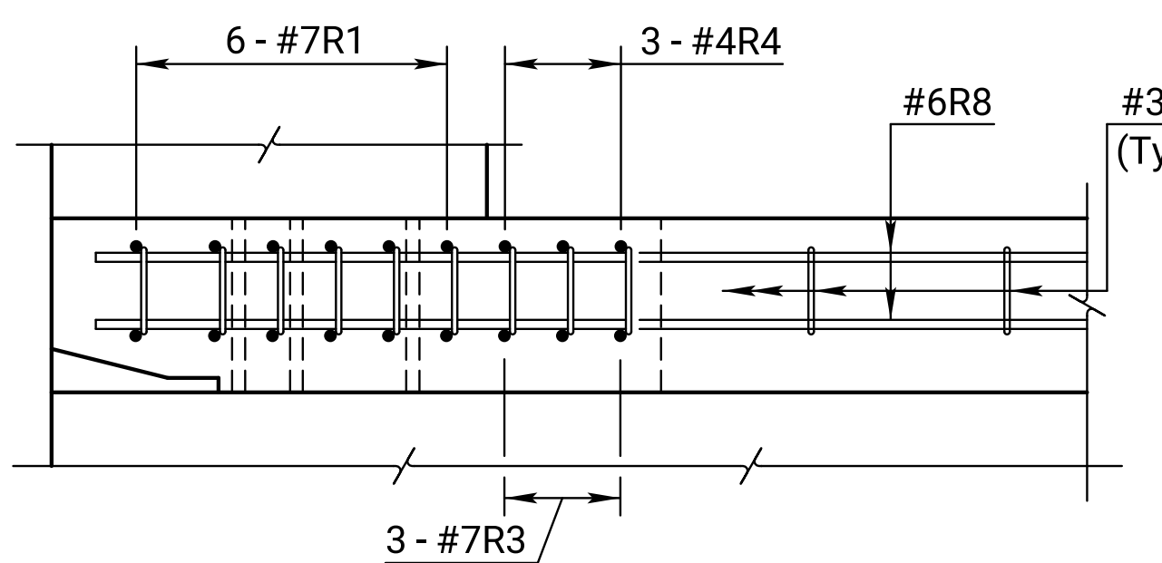
SECTION C-C
