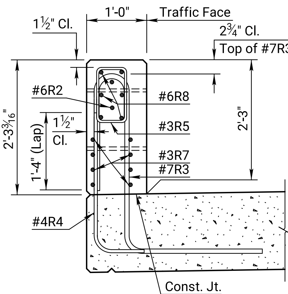
SECTION B-B
