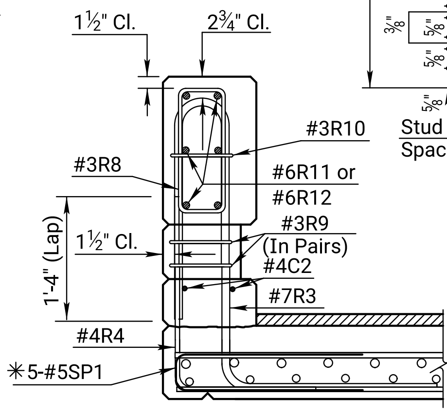
SECTION THRU POST
