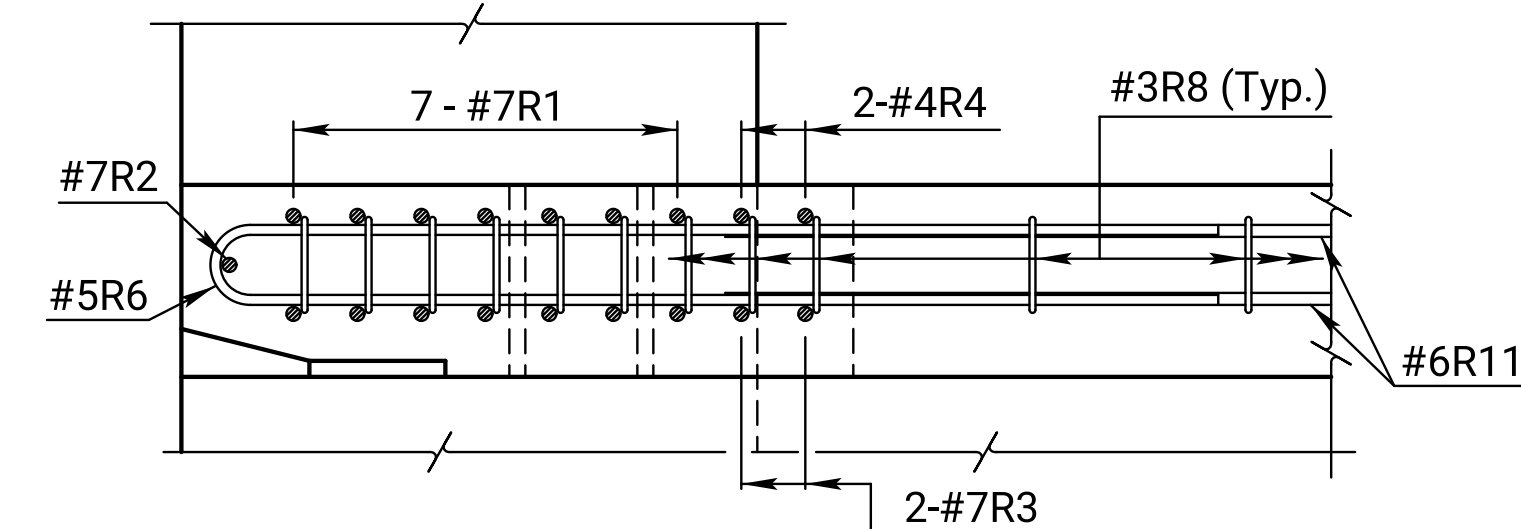
SECTION C-C
