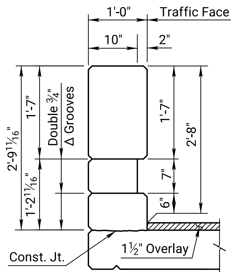
TYPICAL INTERIOR POST
