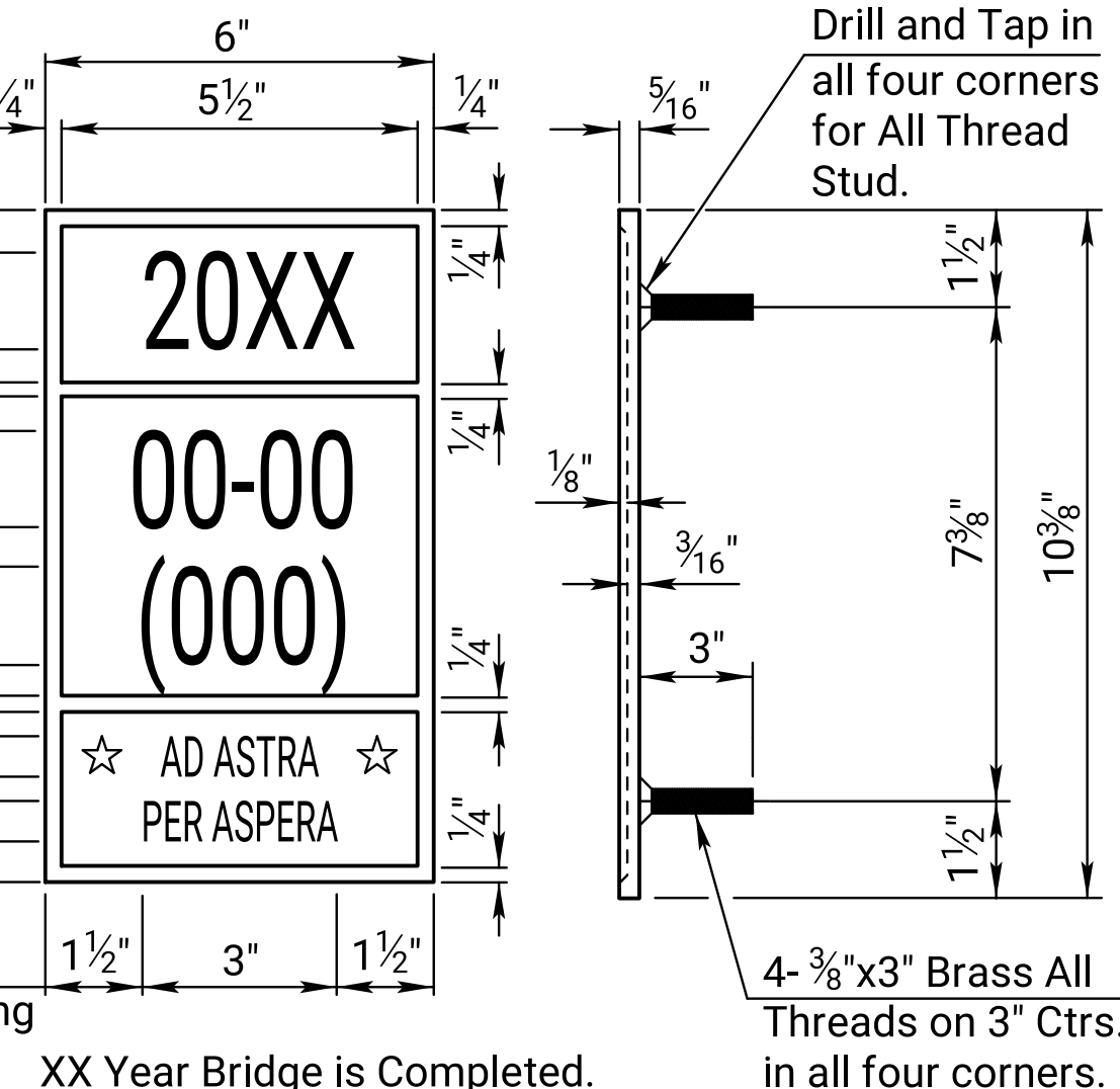
BRIDGE NUMBER PLATE
