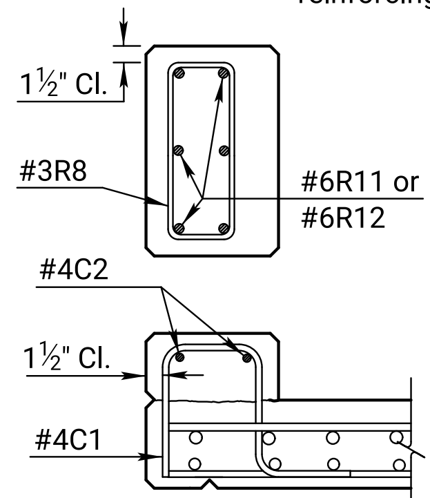
TYPICAL SECTION BETWEEN POSTS
