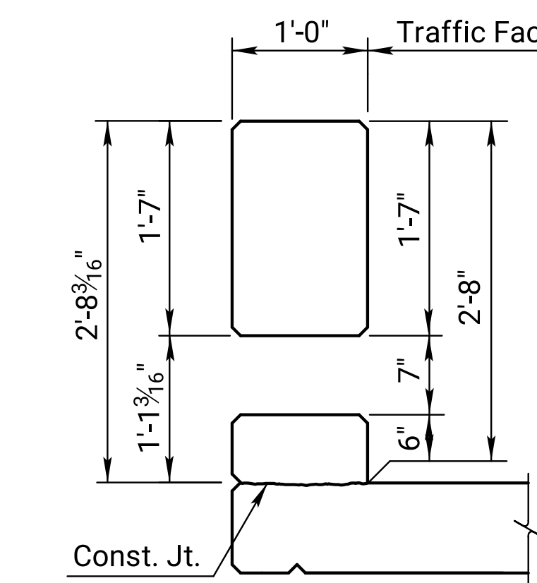
TYPICAL SECTION BETWEEN POSTS
