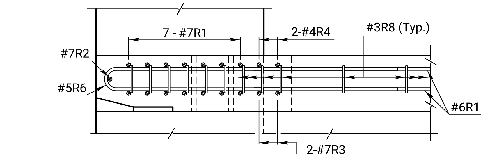
SECTION C-C
