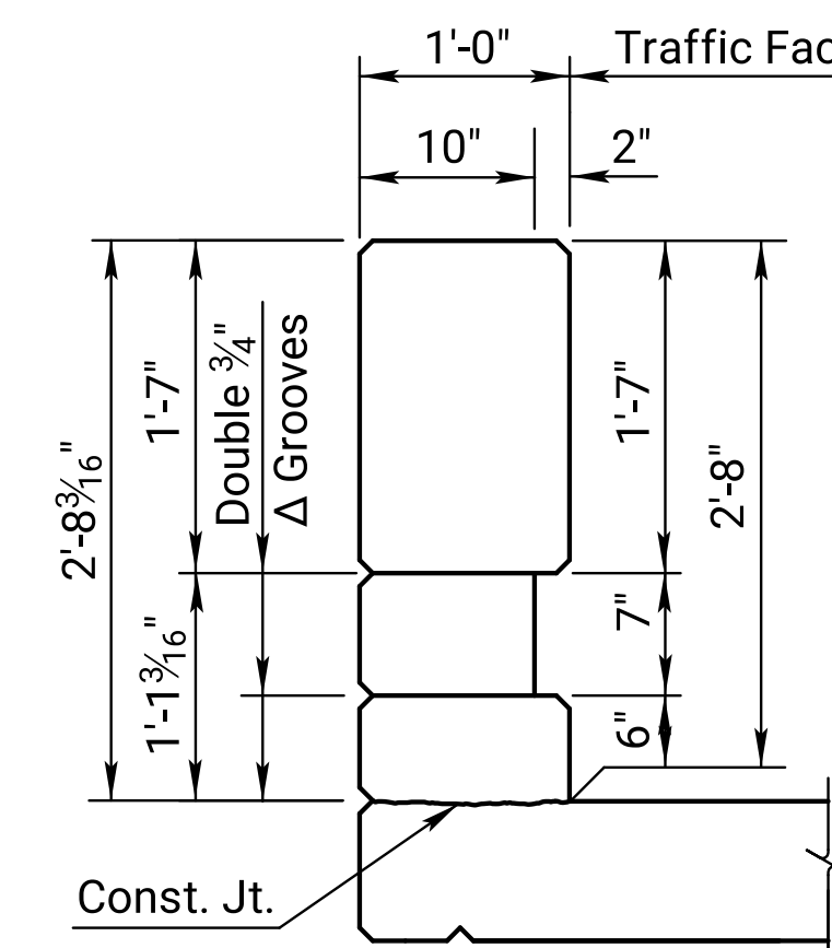
TYPICAL INTERIOR POST
