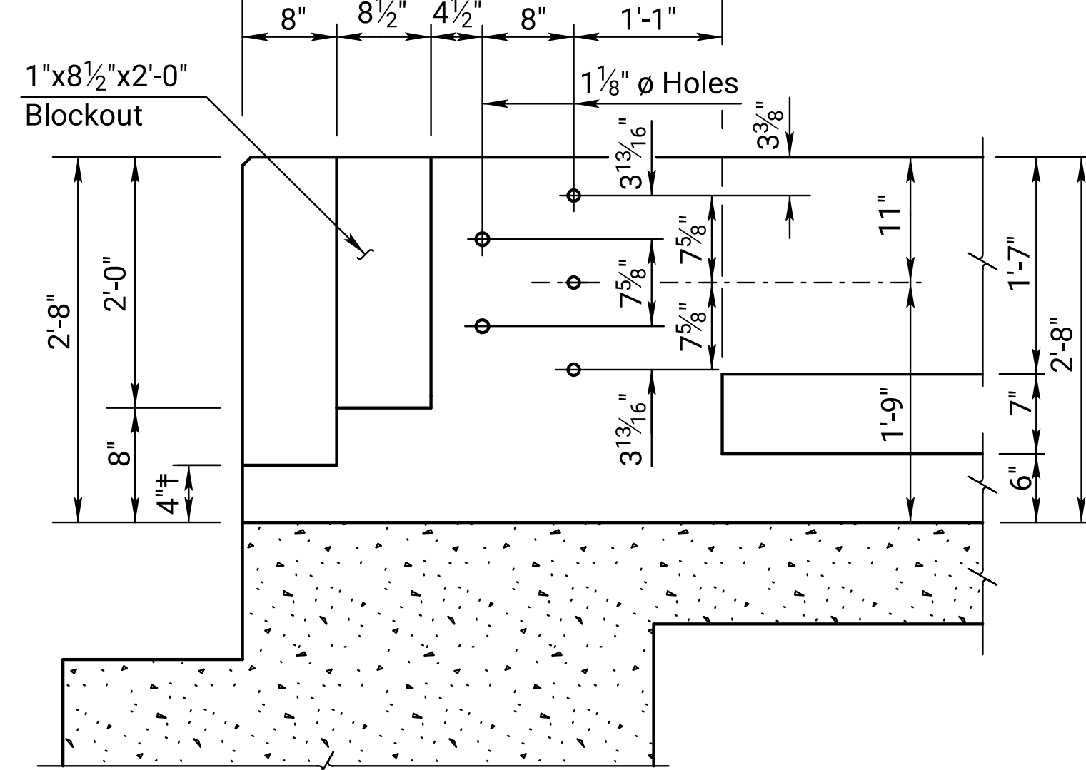
ELEVATION (Dimensions at traffic face of rail.)
