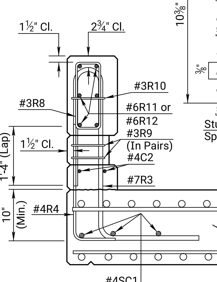
SECTION THRU POST
