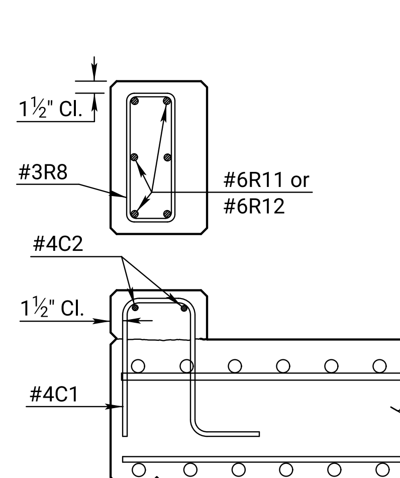
TYPICAL SECTION BETWEEN POSTS
