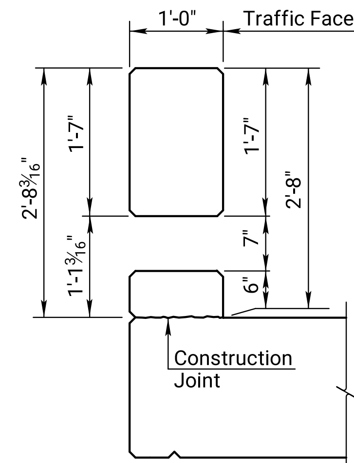
TYPICAL SECTION BETWEEN POSTS
