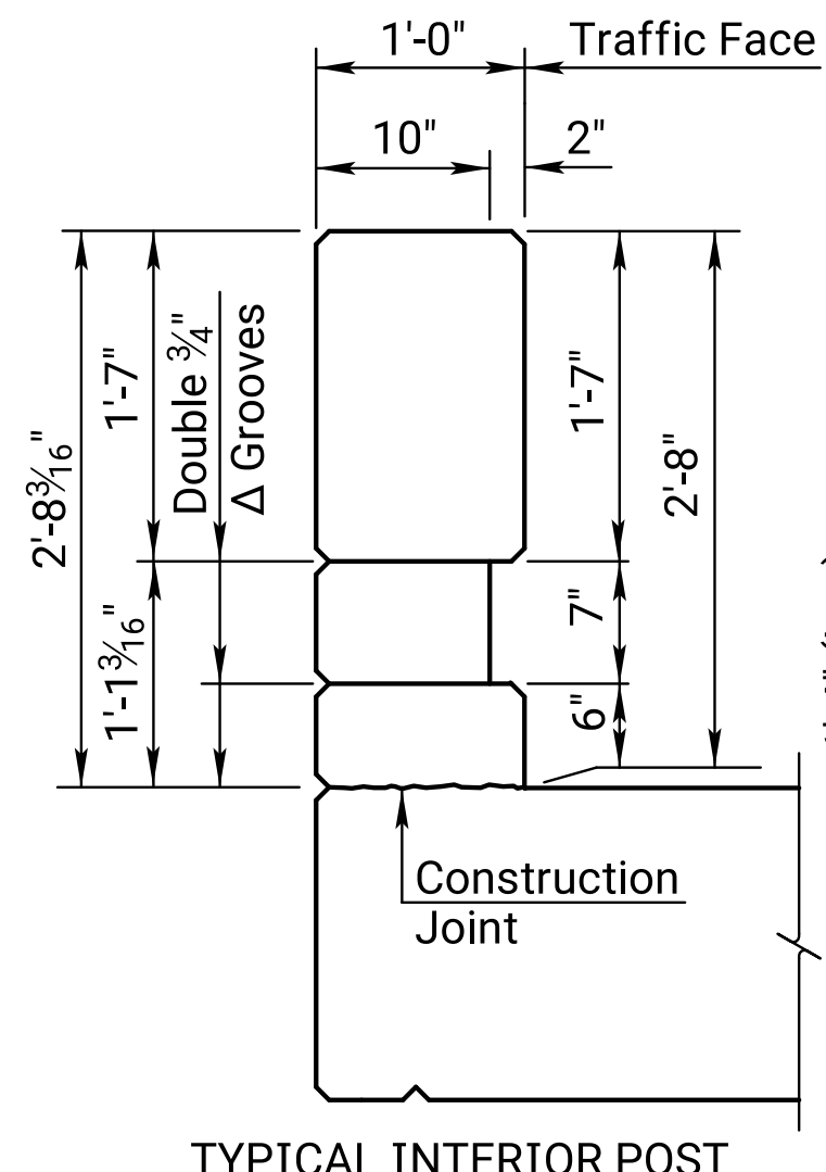
TYPICAL INTERIOR POST
