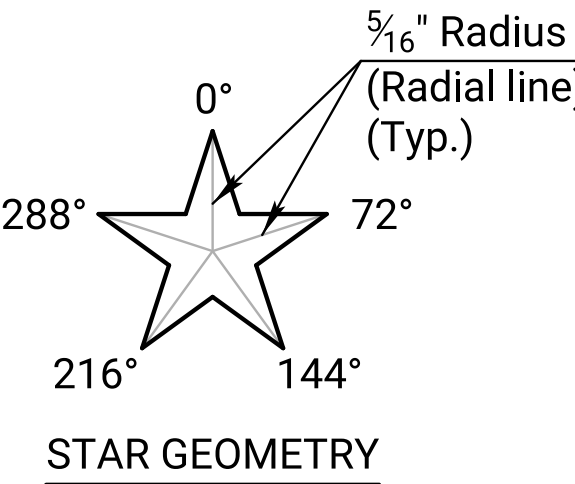
STAR GEOMETRY
