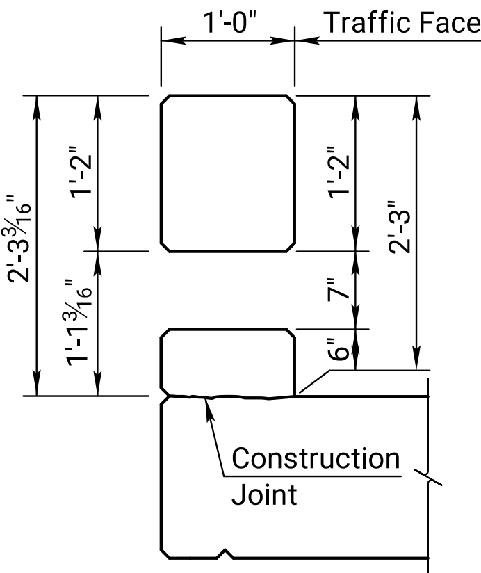
TYPICAL SECTION BETWEEN POSTS
