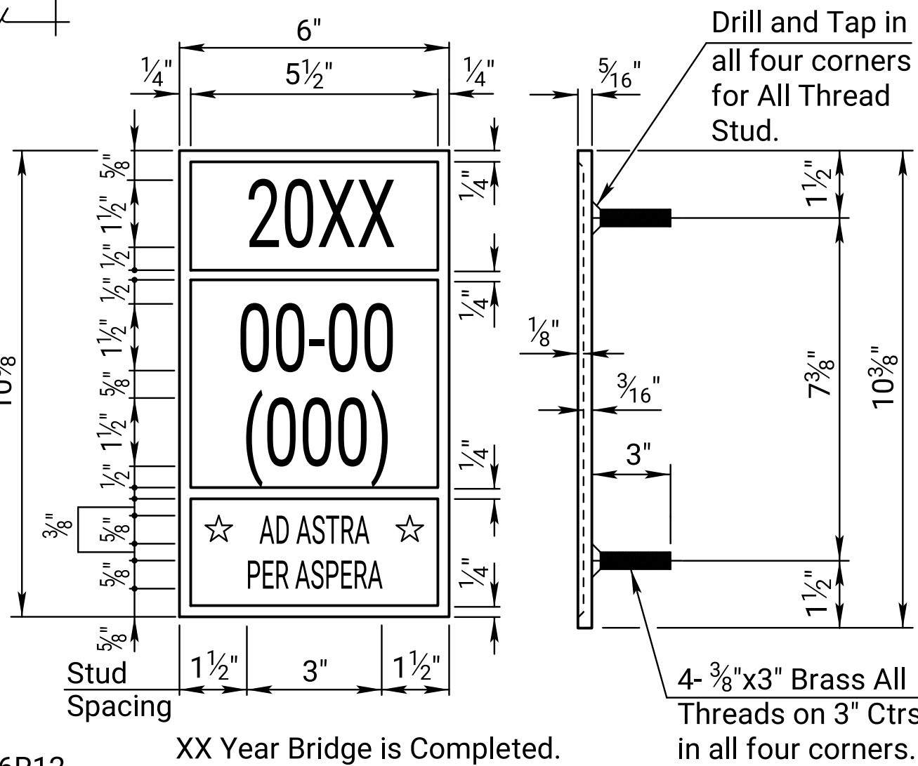
BRIDGE NUMBER PLATE
