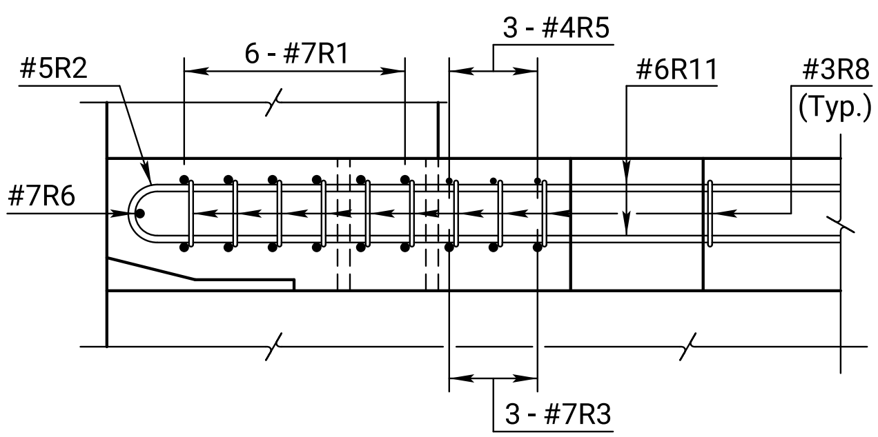
SECTION C-C
